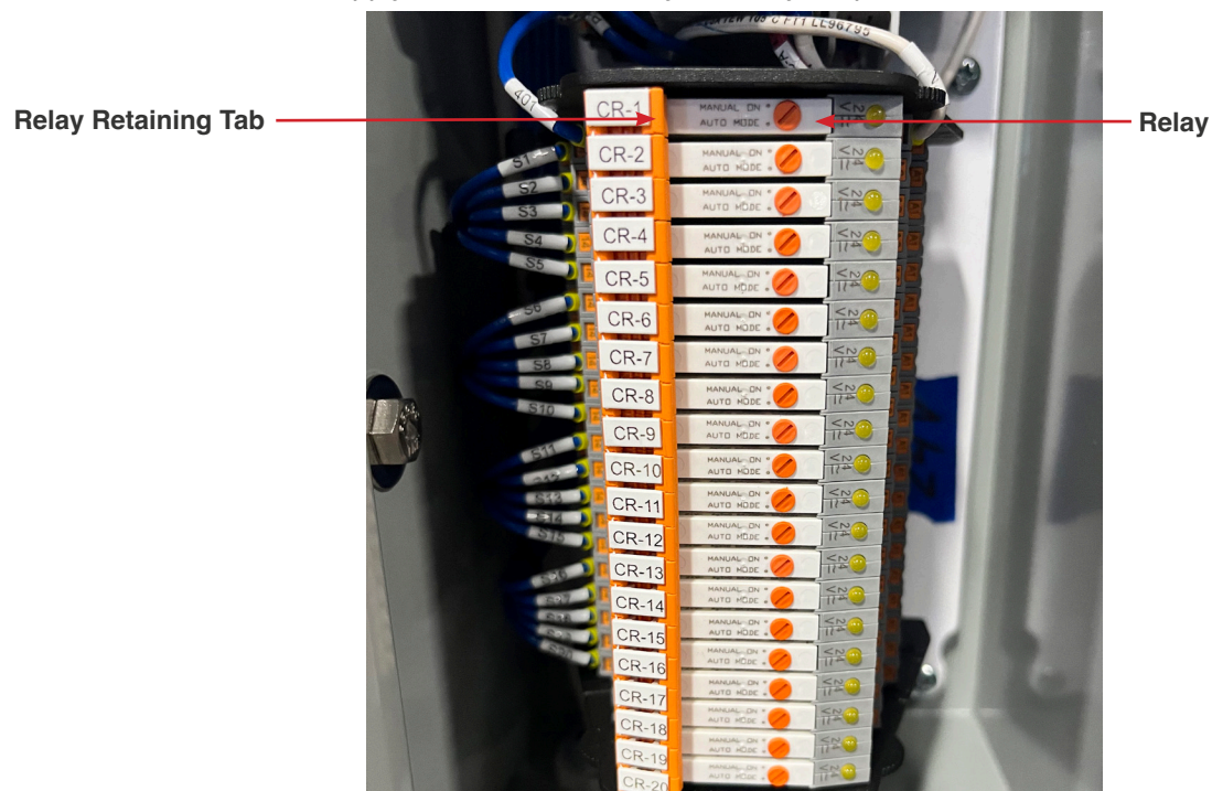
Fig. 7.6 - 1 - Relay replacement
